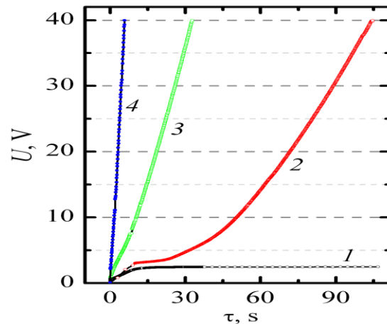
Figure-1. The Ti6Al4V alloy forming dependences obtained in the tartaric acid solutions at j_a , \text{A}\cdot\text{dm}^{-2} : 0.2(1), 0.5(2), 1(3), 5(4). c_A = 50 \text{ g}\cdot\text{dm}^{-3} . The final value of U = 40 \text{ V} .
