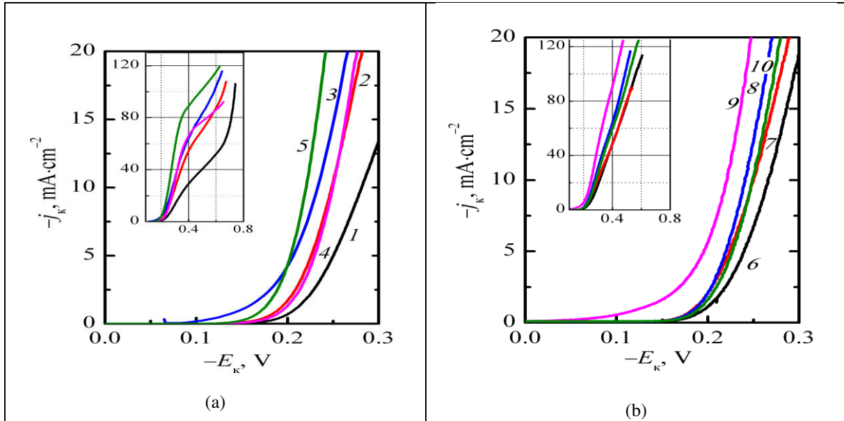
Figure-4. Cathode polarization dependences obtained for the oxidized Ti6Al4V alloy in the sulfate electrolyte: a – dependencies obtained for the specimens oxidized at j_a = 2 \text{ A}\cdot\text{dm}^{-2} , c_A = 50 \text{ g}\cdot\text{dm}^{-3} reaching the final value of U, \text{ V} : 5(1), 10(2), 30(3), 40(4), 50(5); b – the dependences obtained for the specimens oxidized at j_a = 2 \text{ A}\cdot\text{dm}^{-2} , c_A = 50 \text{ g}\cdot\text{dm}^{-3} reaching the final value of U, \text{ V} : 60(6), 70(7), 80(8), 90(9), 100(10).
