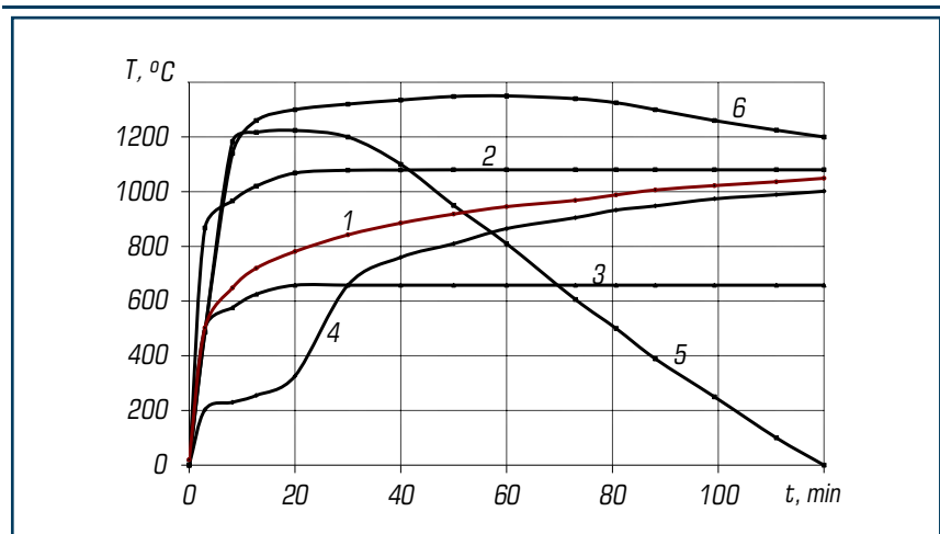
○ Fig. 2.5 Dependence of temperature change on the duration of fire exposure at different heating rates: 1 – standard temperature curve according to ISO 834 and GOST 30247.0-94; 2 – hydrocarbon curve according to EN 1363-2:1999; 3 – minimized a single standard temperature curve according to ISO 834; 4 – external fire curve according to EN 1363-2:1999; 5 – tunnel curve according to German standards (RABT); 6 – tunnel curve according to the standards of the Netherlands (RWS)
