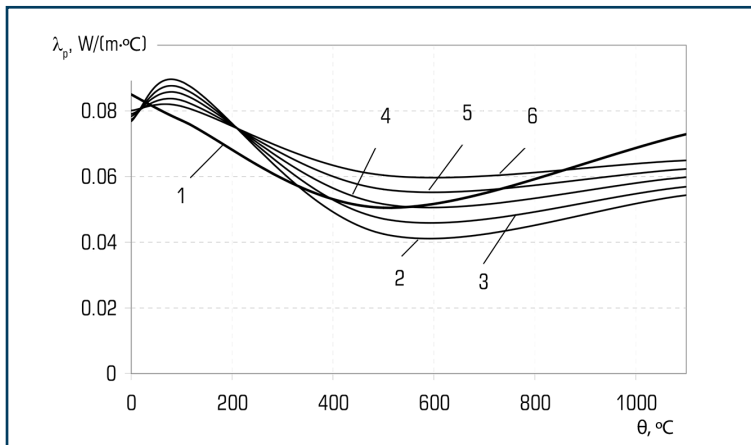
Fig. 5.5 Dependence of the effective coefficient of thermal conductivity of the plaster coating on the temperature found by solving the inverse problems of thermal conductivity according to the data on fire resistance tests: 1 – at \alpha_{c2} , which depends on the temperature; 2 – \alpha_{c2}=3 W/(m 2 ·°C); 3 – \alpha_{c2}=4 W/(m 2 ·°C); 4 – \alpha_{c2}=5 W/(m 2 ·°C); 5 – \alpha_{c2}=6 W/(m 2 ·°C); 6 – \alpha_{c2}=7 W/(m 2 ·°C)
