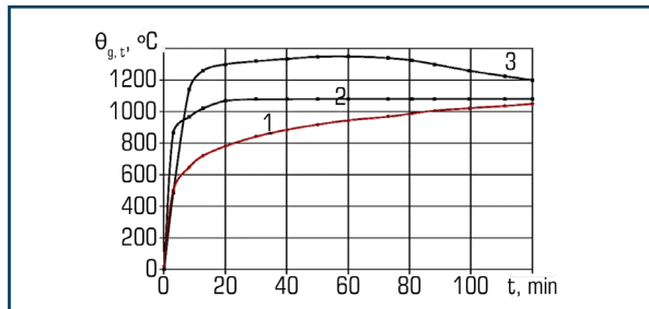
○ Fig. 5.7 Dependence of temperature change on the duration of fire exposure in different fire modes, where: 1 – standard temperature curve according to ISO 834 and GOST 30247.0-94; 2 – hydrocarbon curve according to EN 1363-2:1999; 3 – tunnel curve according to Netherland's standards (RWS)
