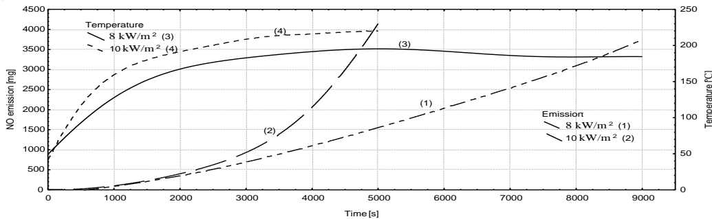
Fig. 4. Average emission of NO from tested specimens and alternation of average temperature
