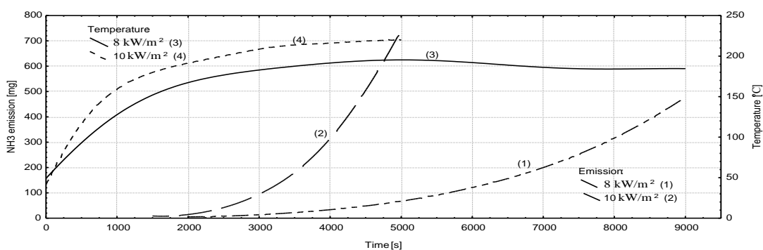
Fig. 7. Average emission of \text{NH}_3 from tested specimens and alternation of average temperature
