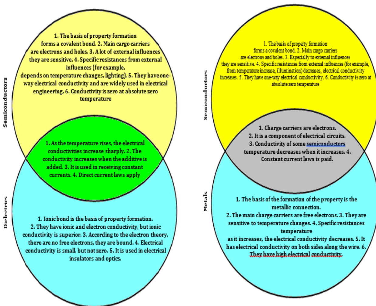
Figure 1. Venn diagram
