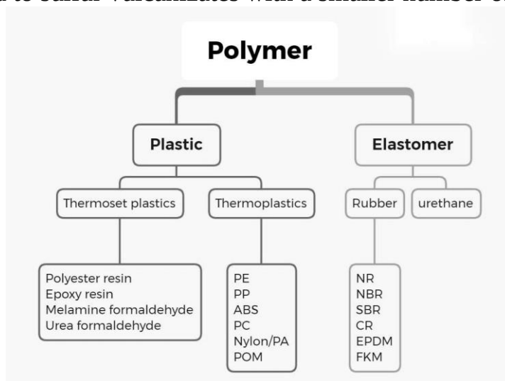
Fig.1. Polymer classification
