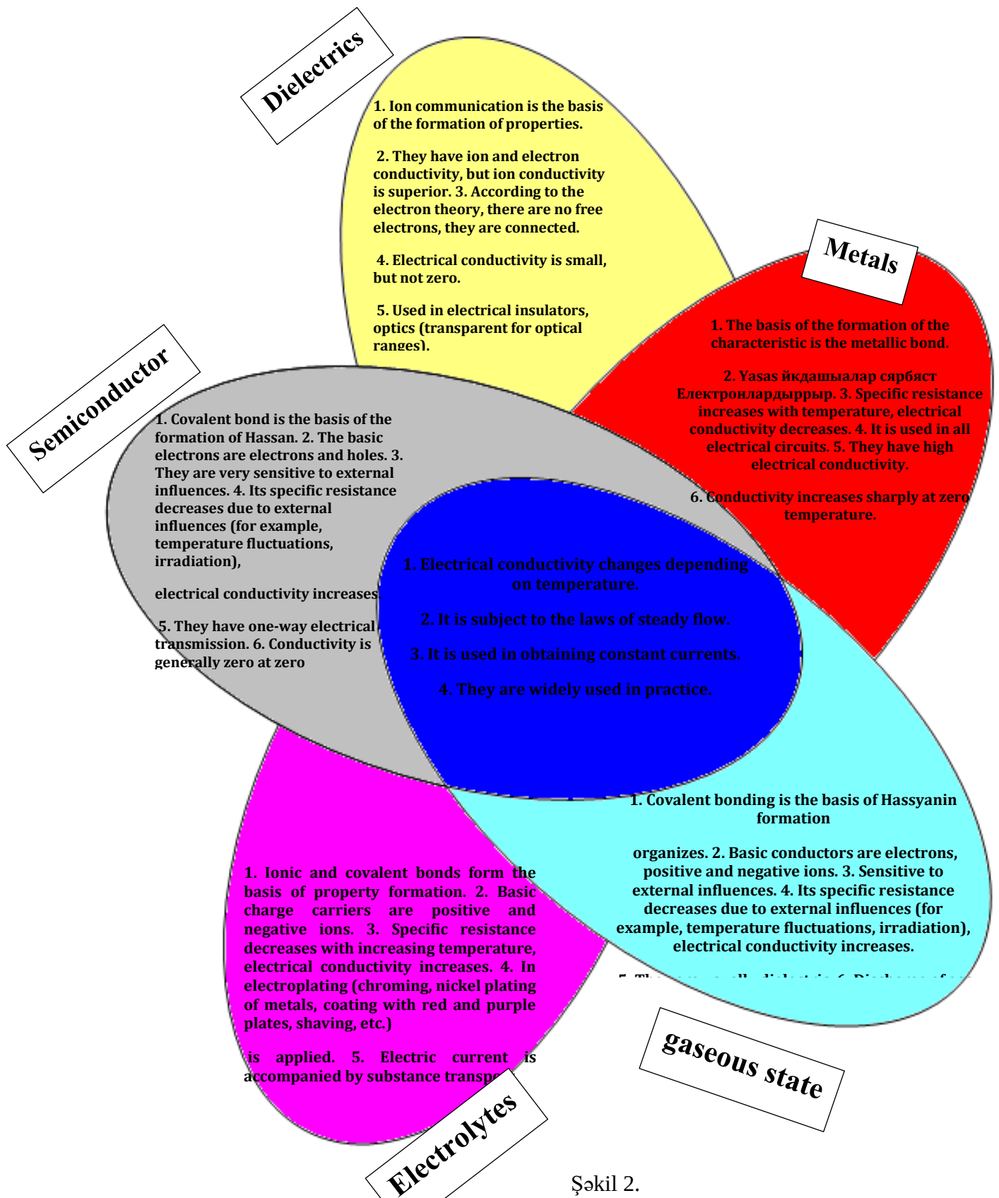
Figure 2. Venn diagram
