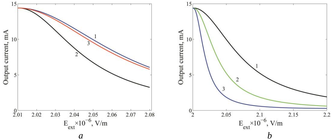
Figure – 3. Dependence of the signal on output of the ring microresonator based on horizontal slot waveguide with the LC filling on electric field intensity.
