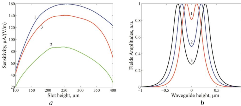
Figure – 4. (a) Dependence of the sensitivity of the sensor on the base of the horizontal slot waveguide with
