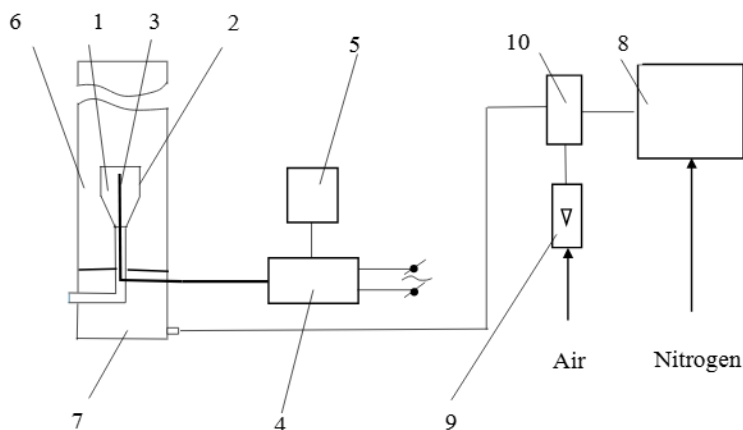
Fig. 2. Diagram of the installation for determining the extinguishing concentration of nitrogen when extinguishing solid combustible substances:
