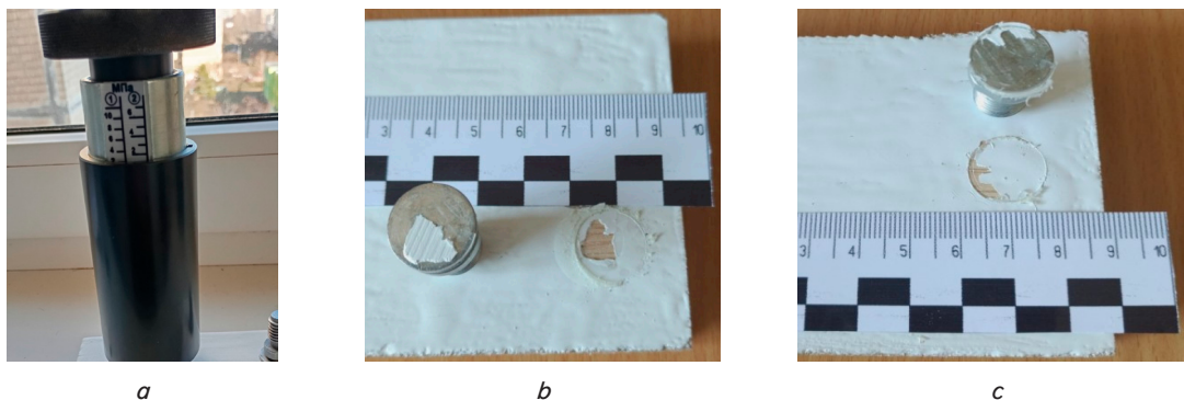
Fig. 3. Results of determining the adhesion strength of the intumescent coating to the samples: a – adhesion research process; b – nature of the stop detachment for wood; c – nature of the stop detachment for particleboard
