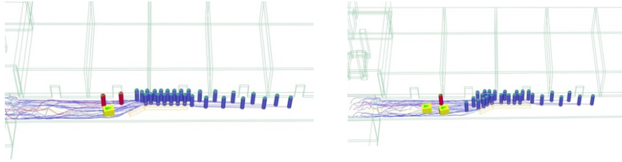
Fig. 7. Computer simulation of the evacuation process
