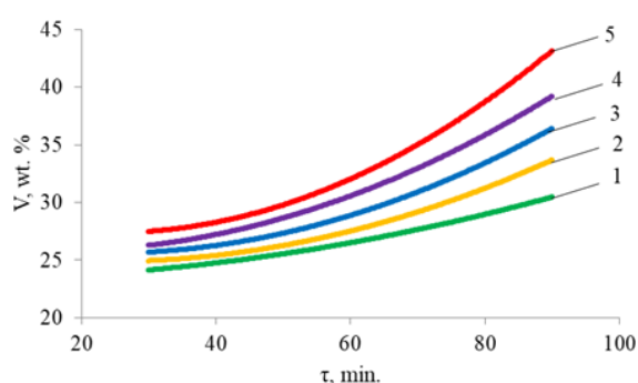
Figure 4. Dependence of V on \tau for the fraction b.p.-180°C (HDPE): 1-P=0.1 MPa; 2-P=0.5 MPa; 3-P=1.0 MPa; 4-P=1.5 MPa; 5-P=2.0 MPa.
