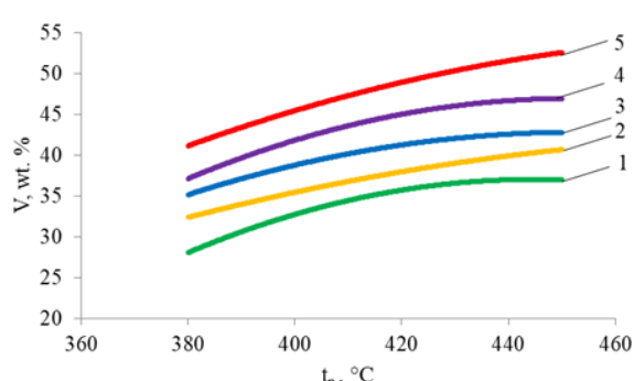
Figure 6. Dependence of V on t_p for the fraction b.p.-180°C (PP): 1-P=0.1 MPa; 2-P=0.5 MPa; 3-P=1.0 MPa; 4-P=1.5 MPa; 5-P=2.0 MPa.
