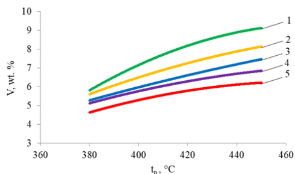
Figure 3. Dependence of V on t_p for gas (HDPE): 1-P=0.1 MPa; 2-P=0.5 MPa; 3-P=1.0 MPa; 4-P=1.5 MPa; 5-P=2.0 MPa.
