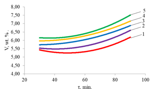
Figure 5. Dependence of V on \tau for gas (HDPE): 1-P=0.1 MPa; 2-P=0.5 MPa; 3-P=1.0 MPa; 4-P=1.5 MPa; 5-P=2.0 MPa.
