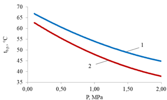
Figure 10. Dependence of t_{b.p.} on P for the fraction b.p.-180°C: 1 – HDPE; 2 – PP.
