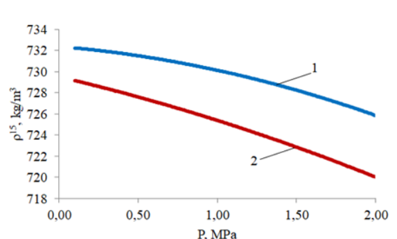
Figure 12. Dependence of \rho^{15} on P for the fraction b.p.-180 °C: 1 – HDPE; 2 – PP.
