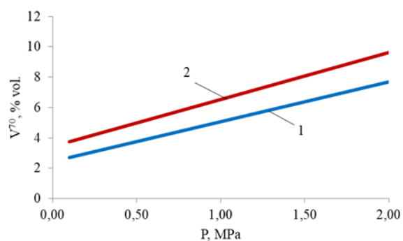
Figure 11. Dependence of V^{70} on P for the fraction b.p.-180°C: 1 – HDPE; 2 – PP.
