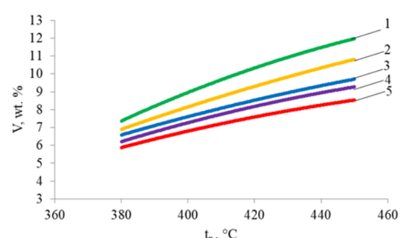
Figure 7. Dependence of V on t_p for gas (PP): 1-P=0.1 MPa; 2-P=0.5 MPa; 3-P=1.0 MPa; 4-P=1.5 MPa; 5-P=2.0 MPa.
