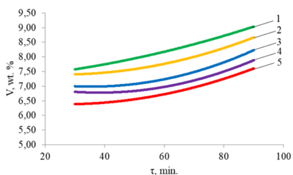
Figure 9. Dependence of V on \tau for gas (PP): 1- P=0.1 MPa; 2- P=0.5 MPa; 3- P=1.0 MPa; 4- P=1.5 MPa; 5- P=2.0 MPa.
