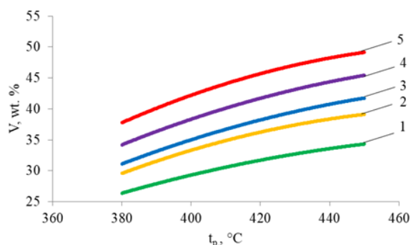
Figure 2. Dependence of V on t_p for the fraction b.p.-180°C (HDPE): 1-P=0.1 MPa; 2-P=0.5 MPa; 3-P=1.0 MPa; 4-P=1.5 MPa; 5-P=2.0 MPa.
