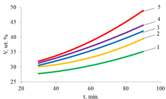
Figure 8. Dependence of V on \tau for the fraction b.p.-180°C (PP): 1- P=0.1 MPa; 2- P=0.5 MPa; 3- P=1.0 MPa; 4- P=1.5 MPa; 5- P=2.0 MPa.
