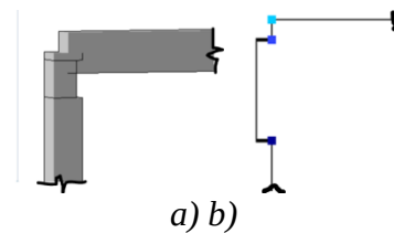
Fig. 2 Fragments of the frame assembly: a) 3- D model; b) analytical model
