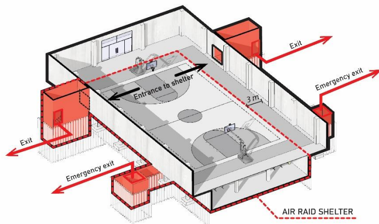
Fig. 1 Scheme of the installation of the shelter under the gymnasium gym hall
