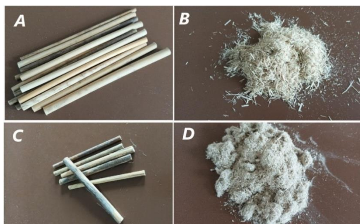
Fig. 1. Photos: A – reed stem waste, B – crushed reed stem waste, C – hemp stem waste, D – crushed hemp stem waste.
