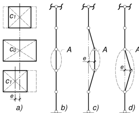
Fig. 1 Column models with symmetrical (asymmetrical) cross-sectional damage
