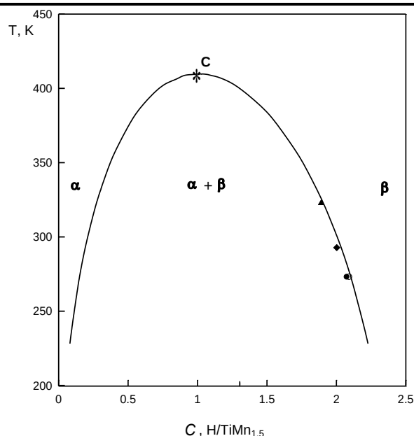
Fig. 1. Decomposition curve of homogeneous phases of the \text{TiMn}_{1.5}\text{-H}_2 system into disordered \alpha -, \beta -phases: — calculation results; *C – critical point of \alpha - \beta -equilibria (calculation); \circ and \bullet, \blacklozenge, \blacktriangle – experimental results on \text{H}_2 desorption.
