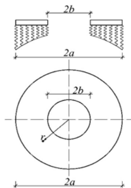
Fig. 1. Annular plate on an inhomogeneous elastic foundation.
