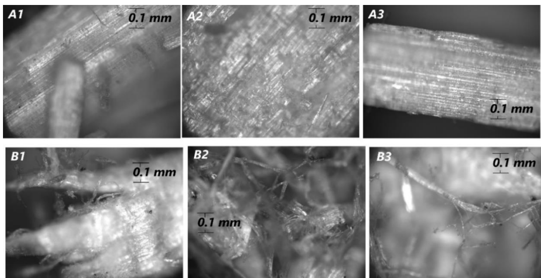
Fig. 2. Microscopic TEM research: A1, A2, A3 –crushed reed stem waste, B1, B2, B3 –crushed hemp stem waste.
