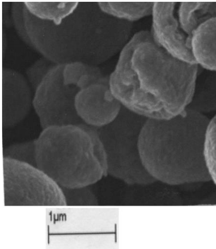
Fig. 1. Hollow deformed microspheres of solid Ti at the bottom of the reactor.
