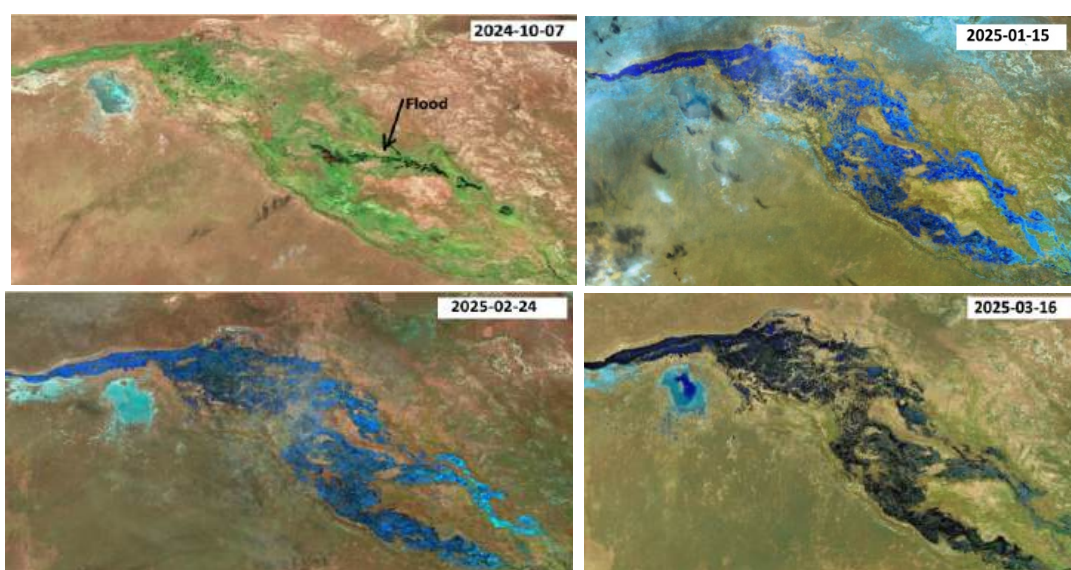
Fig. 3. Flooding regime of the Moyinkum part of the delta region in the warm winter of 2024/2025.
