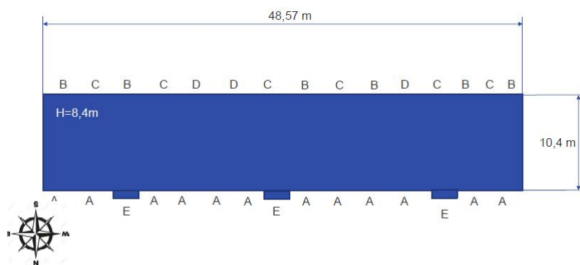
Figure 6 – Window placement and dimensions of the hotel building
