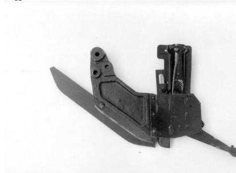
Figure 2. A runner coulters of grain seeder
