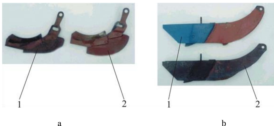
Figure 1. The nature of the wear of vertically placed soil cutting elements of the coulters: a – Suffolk tine point: 1 – worn; 2 – new; b – tine point runner-type: 1 – new; 2 – worn.
