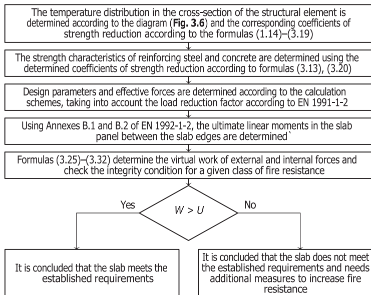
● Fig. 3.20 Scheme of the algorithm for the implementation of the method for the calculated assessment of the fire resistance of the reinforced concrete ribbed slab according to the limit state of the loss of integrity according to the energy criterion
