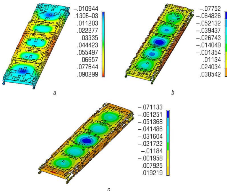
• Fig. 3.13 Distribution of vertical movements ( m ) in the studied reinforced concrete ribbed slab at the time of failure at different levels of the applied active load: a – 30 % of the maximum load; b – 50 % of the maximum load; c – 70 % of the maximum load
