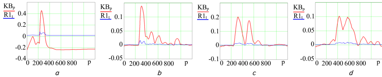
Fig. 1. Dynamics of the difference between KB_r and the threshold R1_r for CO concentration during ignition: a – alcohol; b – paper; c – wood; d – textile
