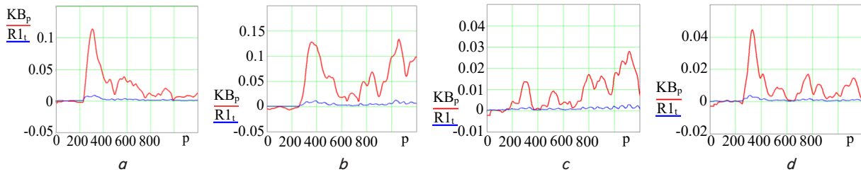
Fig. 3. Dynamics of the difference between KB_r and the threshold R1_r for the ignition temperature: a – alcohol; b – paper; c – wood; d – textiles
