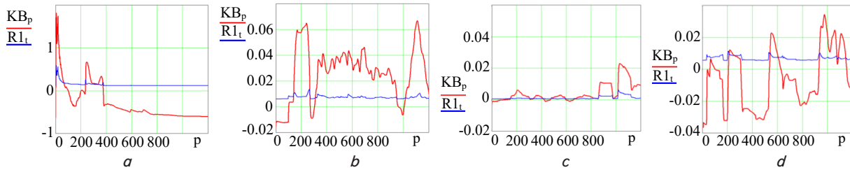
Fig. 2. Dynamics of the difference between KB_r and the threshold R1_r for smoke density during ignition: a – alcohol; b – paper; c – wood; d – textile
