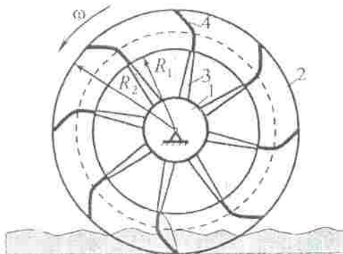
Fig. 3. Scheme of the groundthrower mechanism
