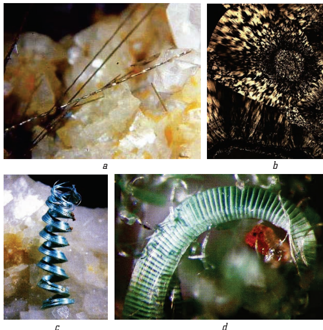
Fig. 3. Crystals grown by a layer-by-layer mechanism: a – malachite crystal; b – chalcedony crystal; c – millerite crystal; d – pyrite crystal
