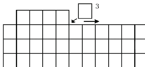
Fig. 2. Two-dimensional crystal growth model
