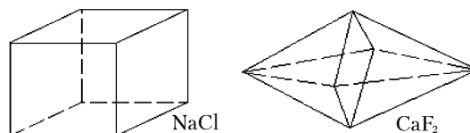
Fig. 5. The equilibrium shape of the crystals of certain compounds
